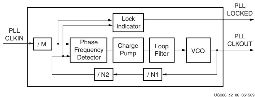
Figure 2-9: PLL Detail
