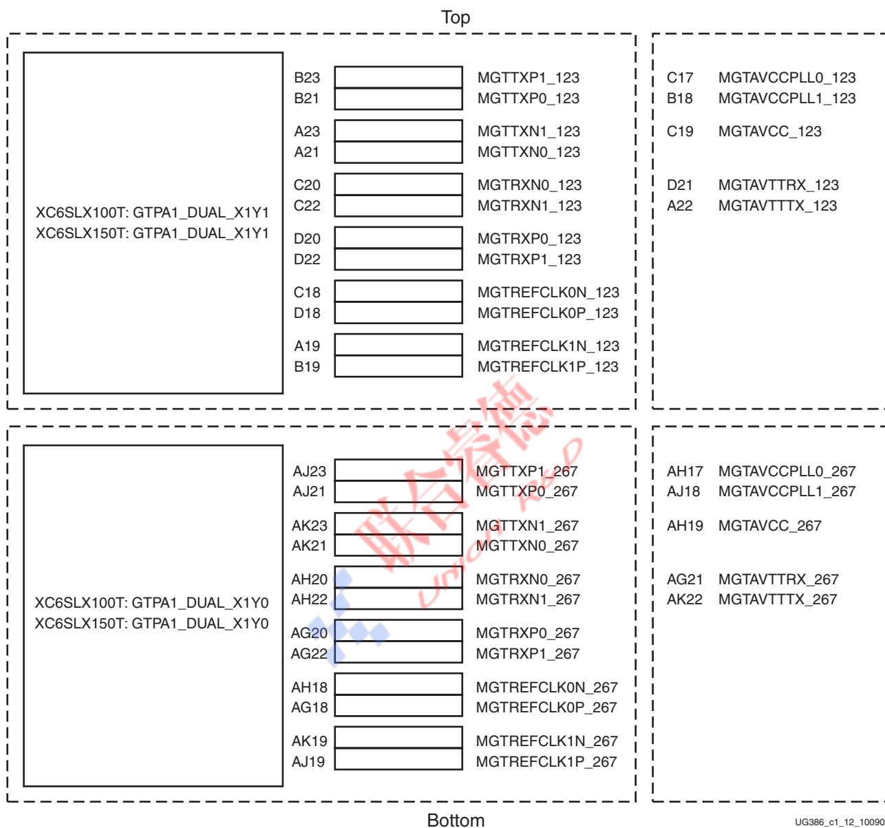
Figure 1-14: Placement Diagram for the FG(G)900 Package (2 of 2)
