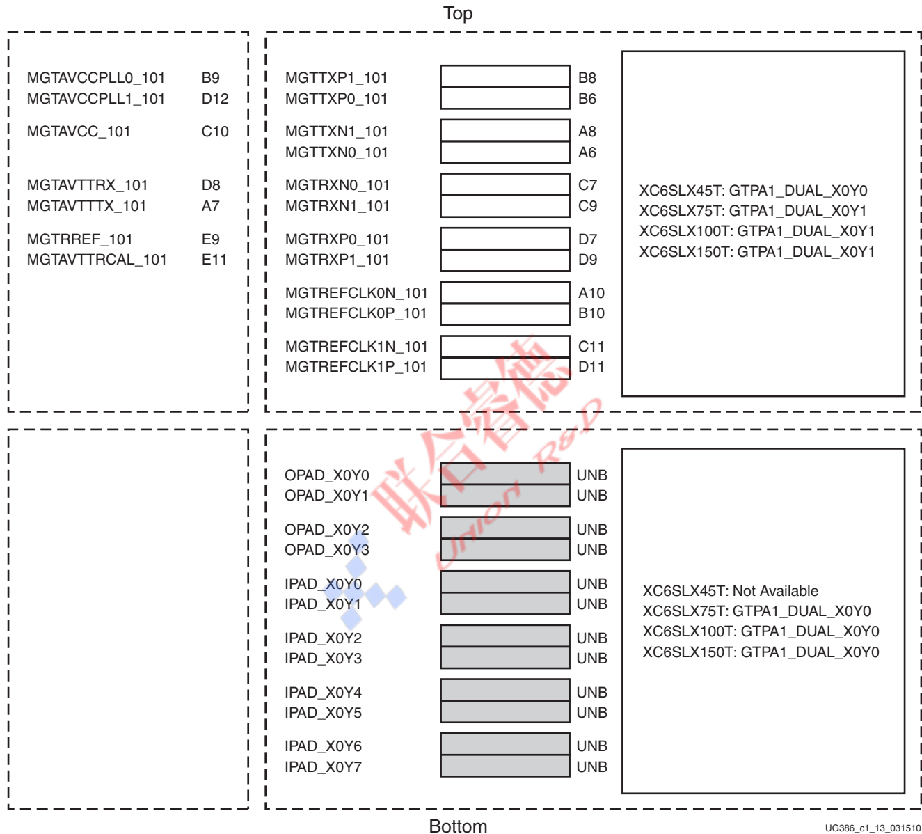
Figure 1-7: Placement Diagram for the CSG484 Package (1 of 2)
