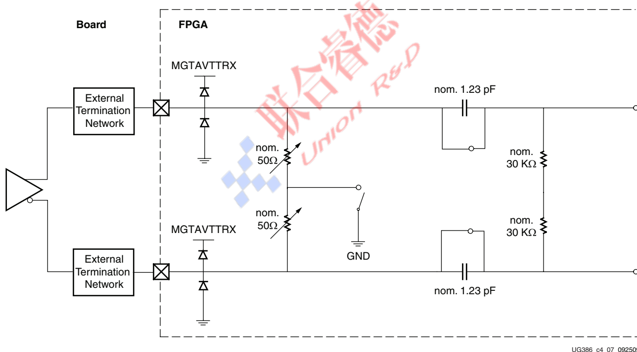
Figure 4-6: RX Termination Use Mode 4 Configuration
