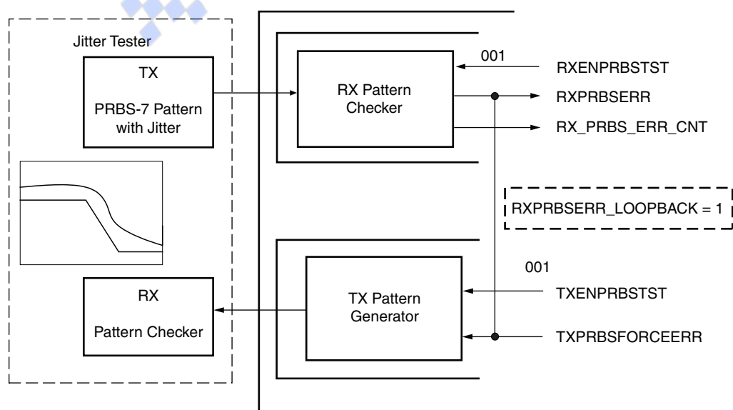
Figure 3-17: Jitter Tolerance Test Mode with a PRBS-7 Pattern
