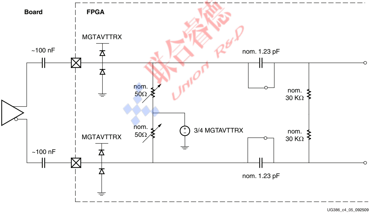
Figure 4-4: RX Termination Use Mode 2 Configuration
